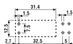
45.91...0310 (1 NO/SPST-NO)
